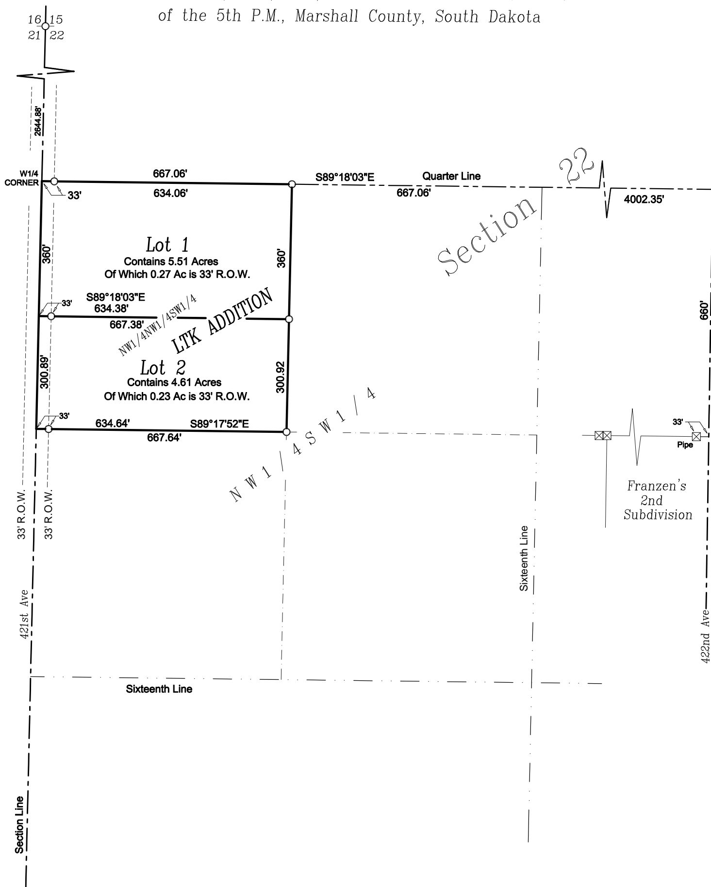
Section Layout
